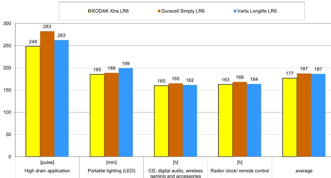
Test Report for Kodak Xtralife AA vs Competitors
